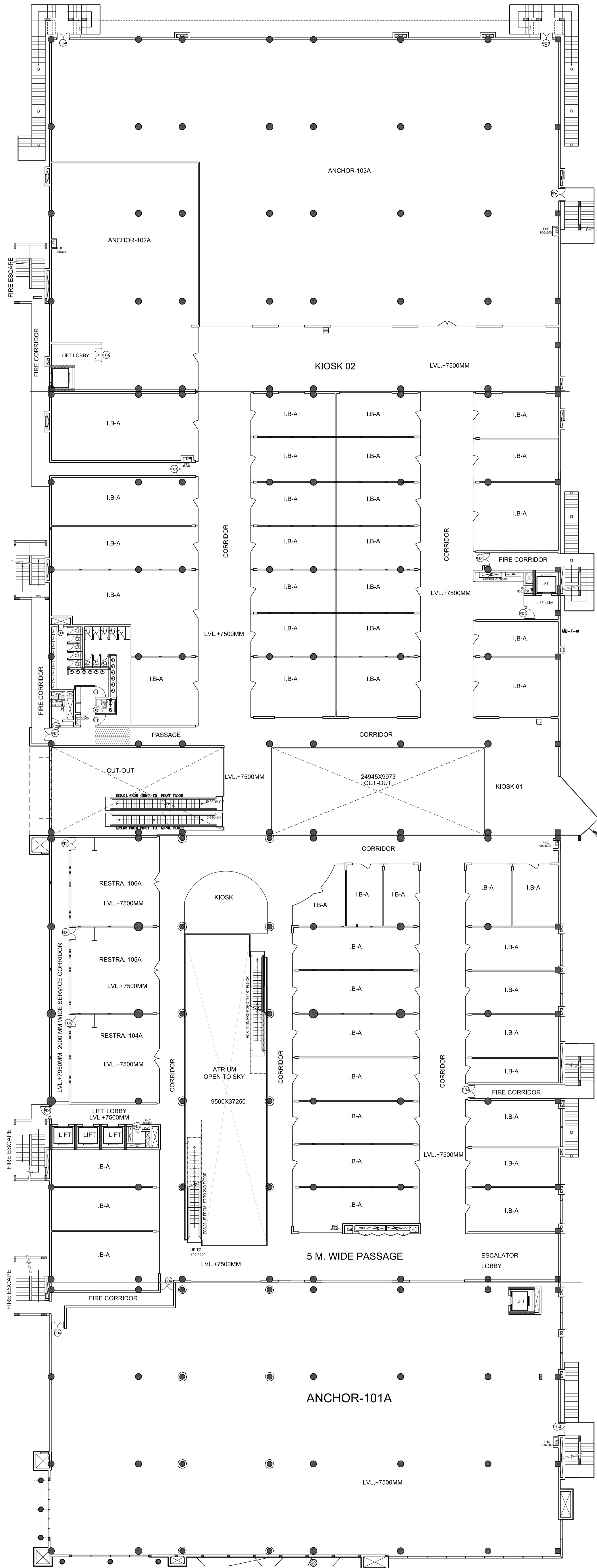
FIRST FLOOR PLAN
